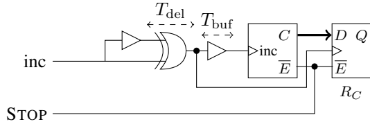
Fig. 8: Solution II: Implementation with look-ahead Gray code counter and register. The counter C is initialized with 1. Register R_C is of same width as the counter, and initialized with 0.
