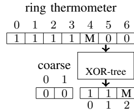
Fig. 10: Circuit encoding a TDC measurement value ( n - 1 thermometer encoded ring latch states and B bit coarse BRGC counter state) as a single BRGC encoded value without losing precision in presence of a metastable input bit. Here n = 8 and B = 2 and the coarse counter is even (decimal 0), i.e., we have to count 1s in latch states. Observe that the final value 0011M correctly encodes decimal 4 or 5, depending on how M resolves.
