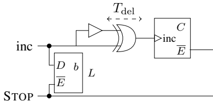
Fig. 12: Solution III: Gray code counter variant with single-bit latch.
