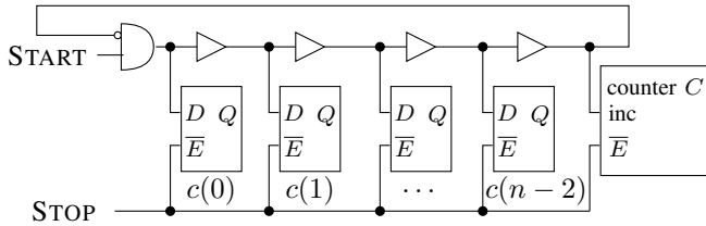
Fig. 2: Generic ring TDC architecture with coarse counter C . Latches and counter are initialized to 0. The counter increments on rising and falling transitions.
