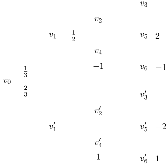
FIGURE 6. An MDP where infinite memory is required for optimal expected value.
