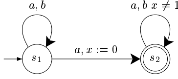
Fig. 1. A non-complementable timed automaton
