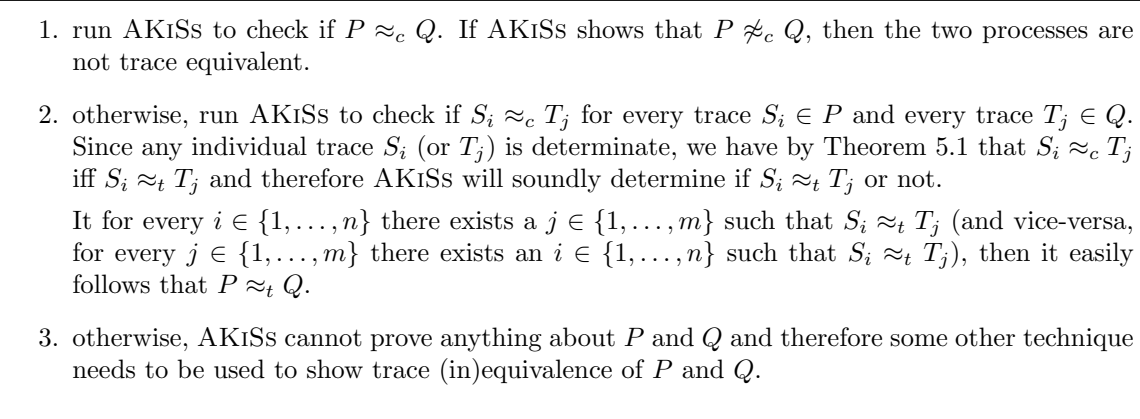
Figure 5.4: How to use AKiSS to check (in)equivalence of processes P = \{S_1, \dots, S_n\} and Q = \{T_1, \dots, T_m\} which are not known to be determinate.
