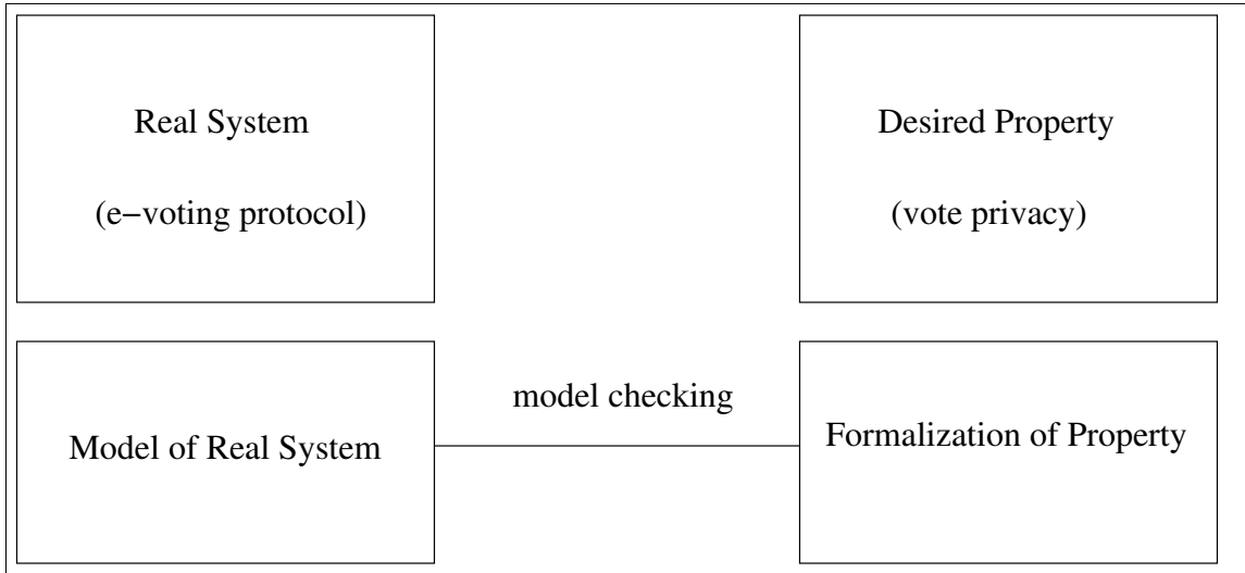
Figure 1.1: Model Checking
