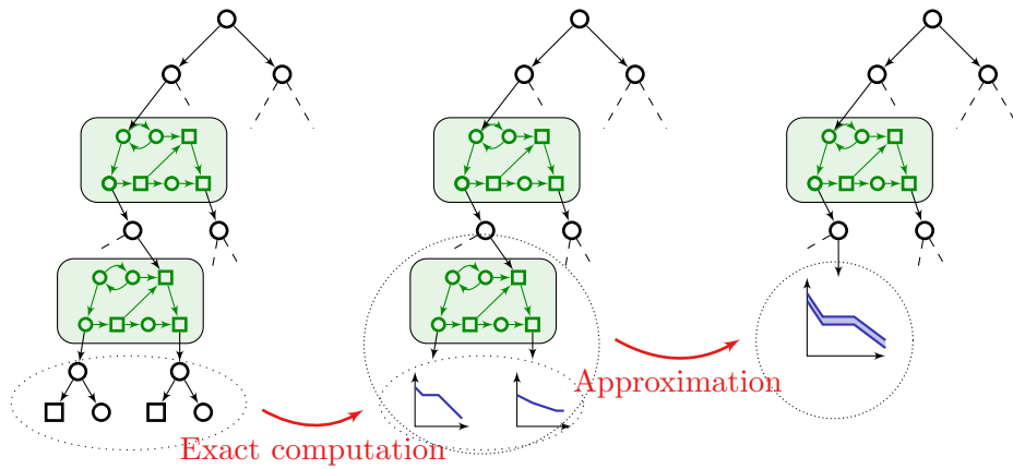
Figure 12: Approximation scheme
