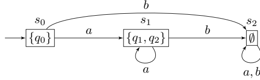
■ Figure 4 The IF-automaton of pLTS of Figure 3.
