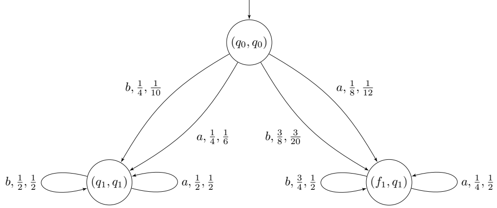
■ Figure 30 Construction of Chen and Kumar for the pLTS of Figure 29
