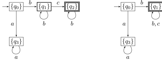
■ Figure 18 On the left a 0-sure predictor of Figure 15, on the right a 1-predictor.
