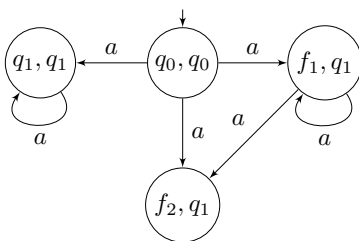
■ Figure 26 The testing sub-pLTS for the pLTS of Fig. 1
