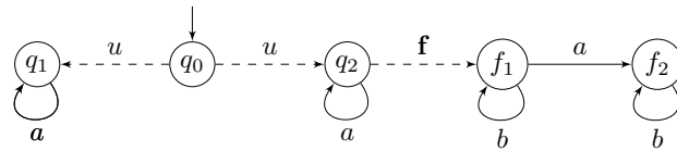
■ Figure 3 A pLTS that is IA-diagnosable but not FA-diagnosable.
