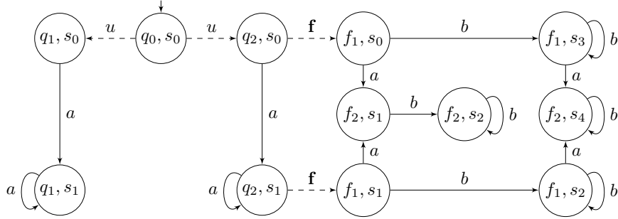
■ Figure 8 The synchronized product of pLTS of Figure 3 and its FA-automaton.
