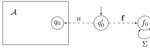
■ Figure 11 A reduction for PSPACE-hardness of IF-diagnosability.
