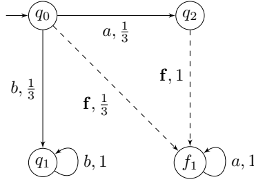
■ Figure 22 A non-predictable pLTS, for which a sure prediagnoser is quicker than all diagnosers.
