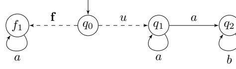
■ Figure 27 A pLTS which is not A-diagnosable
