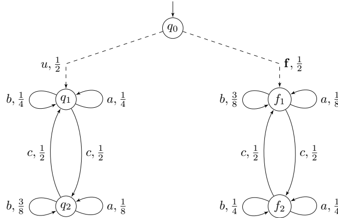
■ Figure 31 Another pLTS which is AA-diagnosable w.r.t. Definition 62.
