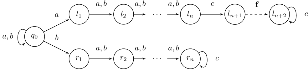
■ Figure 19 A family of 0-surely predictable pLTS requiring predictors with exponential size.
