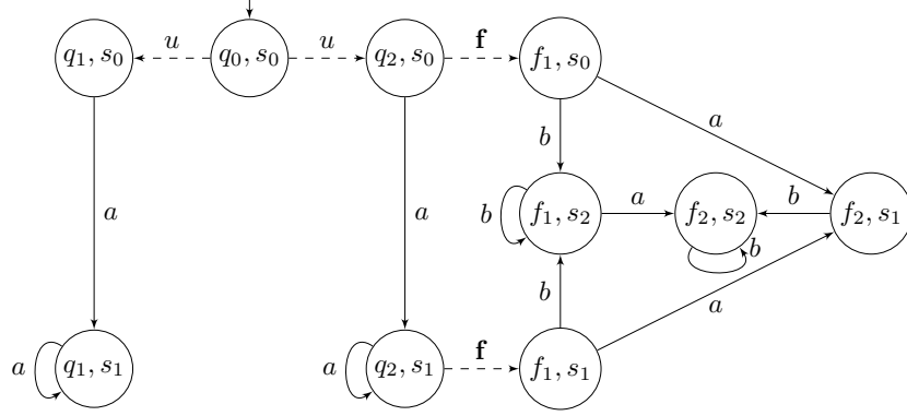
■ Figure 5 The synchronized product of pLTS of Figure 3 and its IF-automaton.
