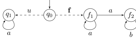
■ Figure 1 A pLTS which is IF-diagnosable but not IA-diagnosable.
