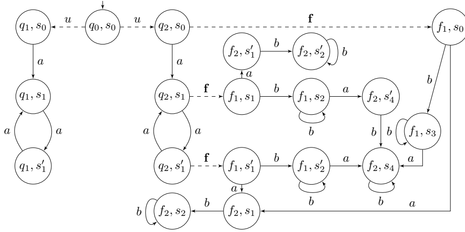
■ Figure 10 The synchronized product of pLTS of Figure 3 and its IA-automaton.
