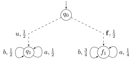
■ Figure 29 A pLTS which is not diagnosable w.r.t. Definition 59 but diagnosable w.r.t. Definition 62.
