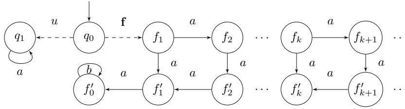
■ Figure 6 An infinite IF-diagnosable pLTS.
