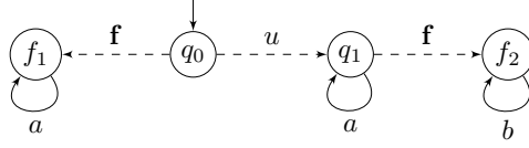
■ Figure 21 A pLTS which is prediagnosable but not IF-diagnosable.
