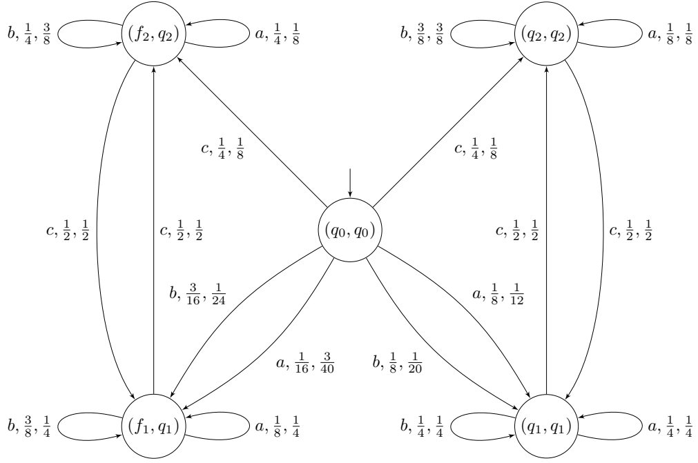
■ Figure 32 Construction of Chen and Kumar for the pLTS of Figure 31
