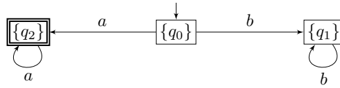
■ Figure 24 A prediagnoser for the pLTS of Figure 23.
