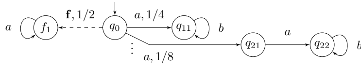
■ Figure 2 An infinitely branching pLTS that is IA- and IF-diagnosable but not FF-diagnosable.
