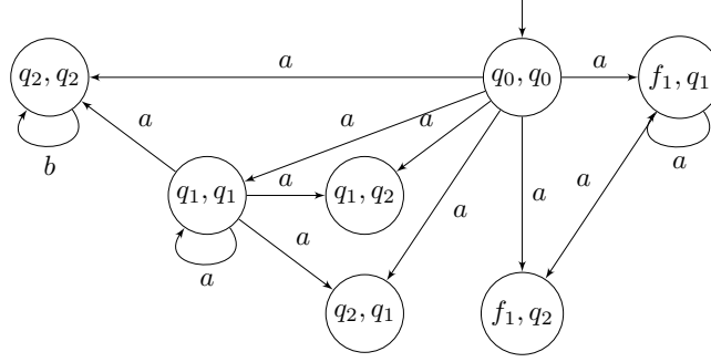
■ Figure 28 The testing sub-pLTS for the pLTS of Fig. 27
