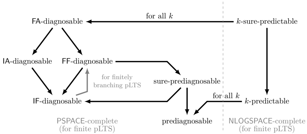
Figure 25 Summarizing relations between specifications, and associated complexities.
