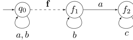
■ Figure 14 A pLTS which is IA-diagnosable.
