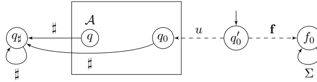
■ Figure 12 A reduction for PSPACE-hardness of FA- and IA-diagnosability.
