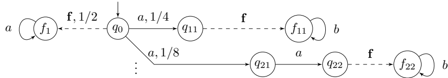
■ Figure 20 An infinitely branching pLTS that is surely prediagnosable but not FF-diagnosable.
