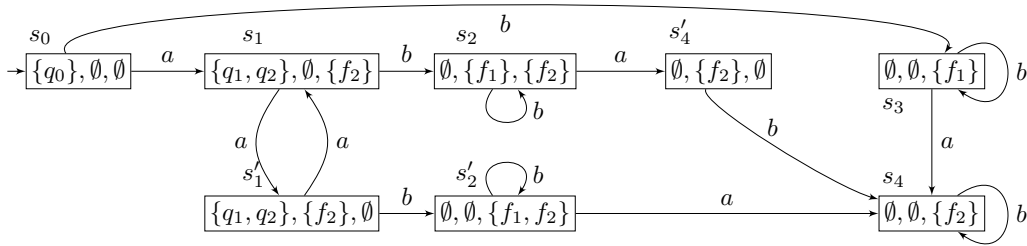
■ Figure 9 The IA-automaton of pLTS of Figure 3.
