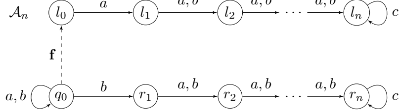
■ Figure 13 Example of an IF-diagnosable pLTS requiring an IF-diagnoser with exponential size.
