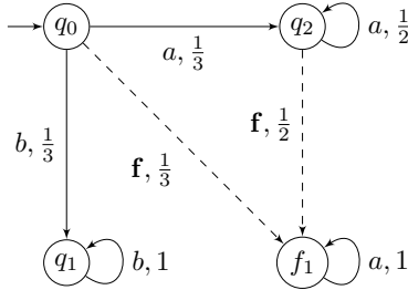
■ Figure 23 A non-predictable, non-diagnosable yet prediagnosable pLTS.
