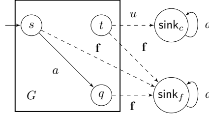
■ Figure 17 Reduction of the reachability problem.
