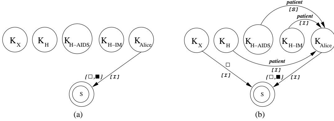
Figure 3. (a) Automaton representing the configurations S = \{\langle K_{\text{Alice}}, \square \rangle, \langle K_{\text{Alice}}, \blacksquare \rangle\} . (b) Automaton representing the configurations in \text{pre}^*(S) .
