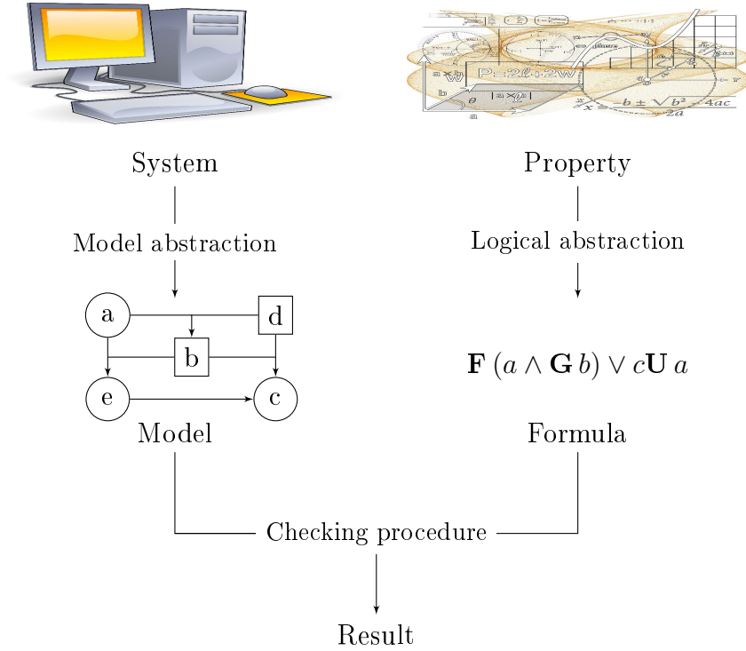
Figure 1: Model checking
