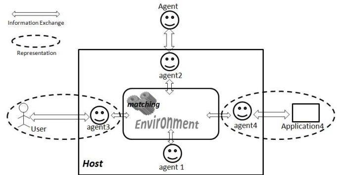
Fig. 1. LACIOS Architecture
