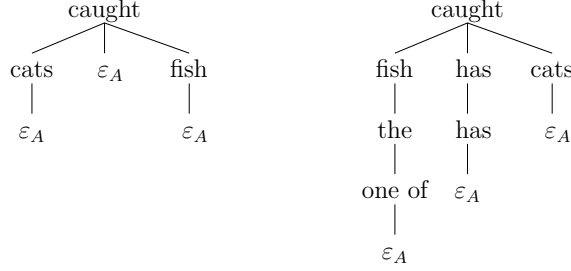
Figure 3: Some trees generated by the regular tree grammar of Example 2.
