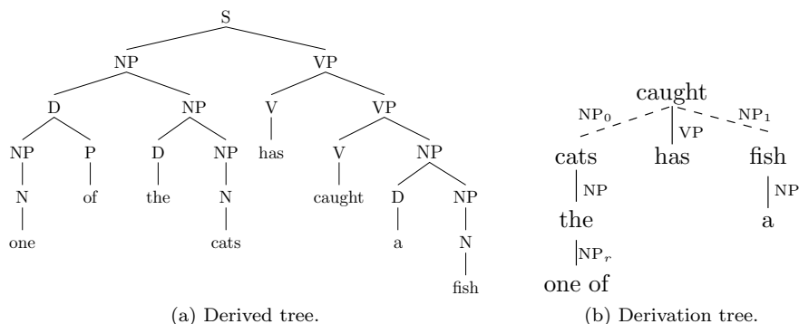
Figure 1: Parse trees for “One of the cats has caught a fish.” using the grammar of Figure 2.
