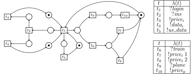
Fig. 2 I/O Petri net of the travel agency
