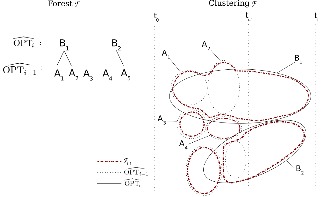
Figure 1: An example of a forest \mathcal{F} given in left, and the corresponding clustering given in right. Here, we have \widehat{\text{OPT}}_i = \{B_1, B_2\} and \widehat{\text{OPT}}_{i-1} = \{A_1, \dots, A_5\} .
