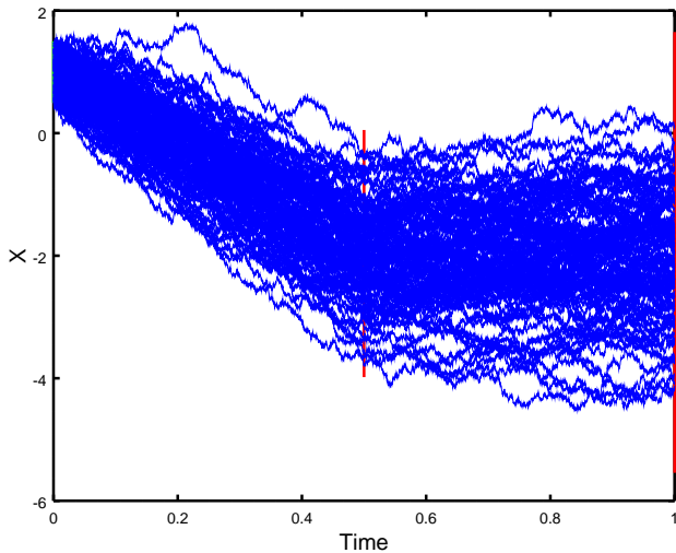
Fig. 8. Example 3 with control pattern (-6, 0) ; initial ball B(z, \delta_0) with z = 1 and \delta_0 = 0.5 ; intermediate ball B(z_1, \delta_1) (at t = \tau = 0.5 ) with z_1 = -2, \delta_1 = 2 ; final ball B(z_2, \delta_2) (at t = 2\tau ) with z_2 = -2, \delta_2 = 3.6
