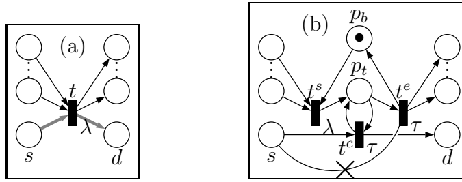
Fig. 3. How to transform a PN+T (a) into a PN+R (b). The edge bearing a \times links the (source) place to be reset to the extended transition. p_{Tr} is not shown.
