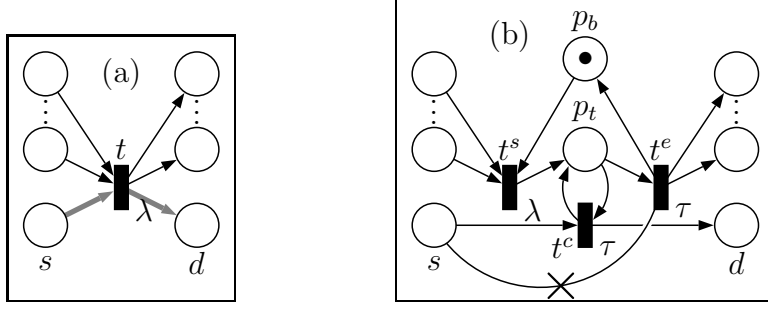
Fig. 4. How to transform a PN+T (a) into a PN+R (b). On this figure, we have adapted a conventional graphical convention to represent reset arcs: the arc bearing a \times links the (source) place to be reset to the extended transition and p_{Tr} (irrelevant in this case) is not shown.
