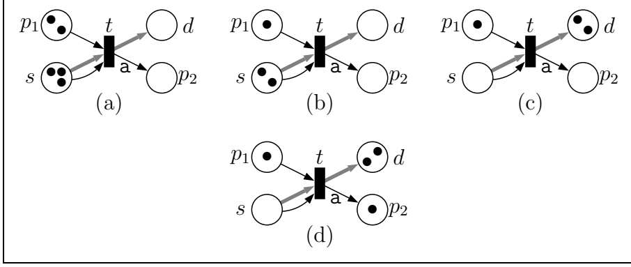
Fig. 1. The four steps to compute the effect of a transfer arc
