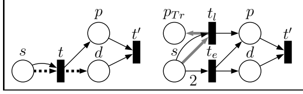
Fig. 2. A PN+NBA \mathcal{N} (a) and the corresponding PN+T \mathcal{N}' (b)
