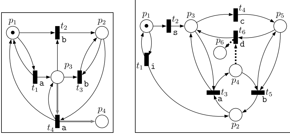
Fig. 3. (a) The PN+T \mathcal{N}_1 and (b) the PN+NBA \mathcal{N}_2 .
