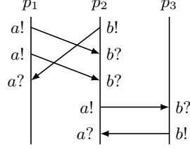
Fig. 1. An MSC with 3 processes
