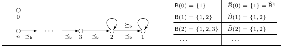
Fig. 1. Backward reachability with \text{Final} = \{1\} .
