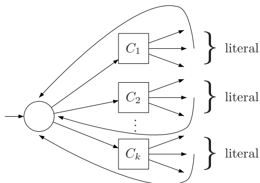
■ Figure 3 Game graph construction for a 3SAT formula (Lemma 12).
