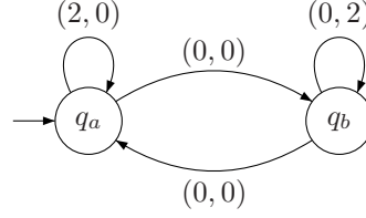
■ Figure 2 A generalized mean-payoff game where infinite memory is necessary to win (Lemma 7).
