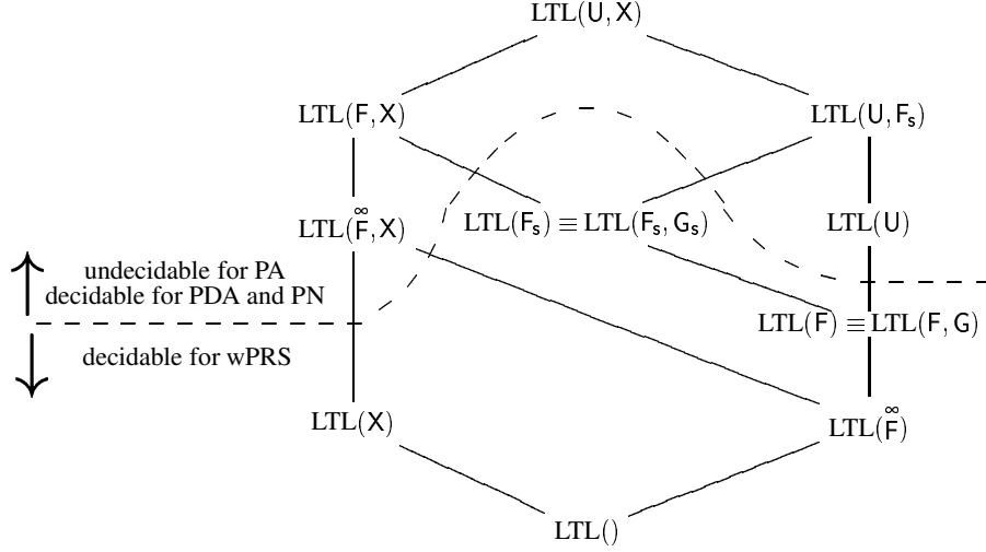
Fig. 2. The hierarchy of basic fragments with model checking decidability boundary.
