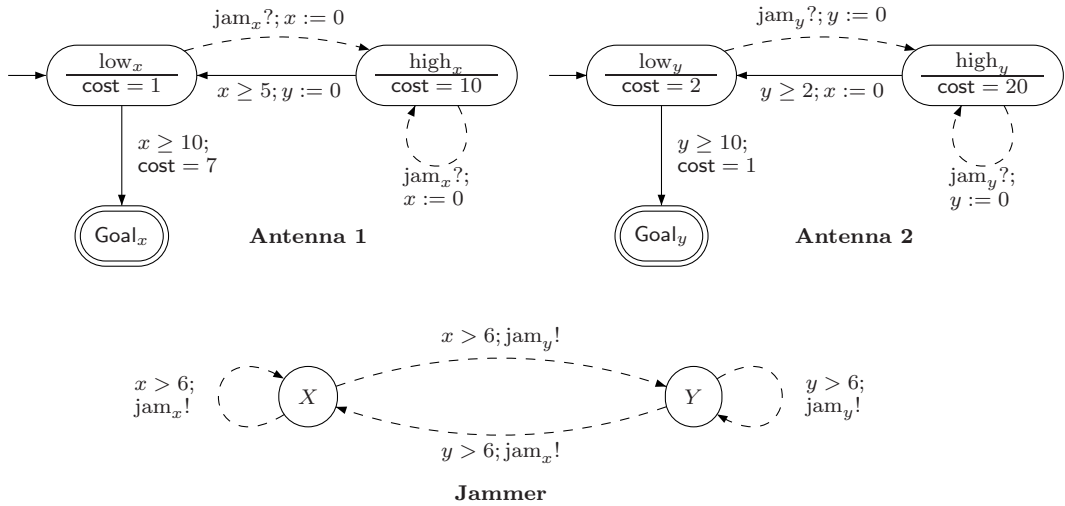
Fig. 8. Mobile Phone Example.
