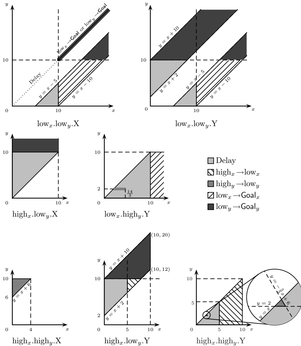
Fig. 9. Optimal Strategy for the Mobile Phone Example
