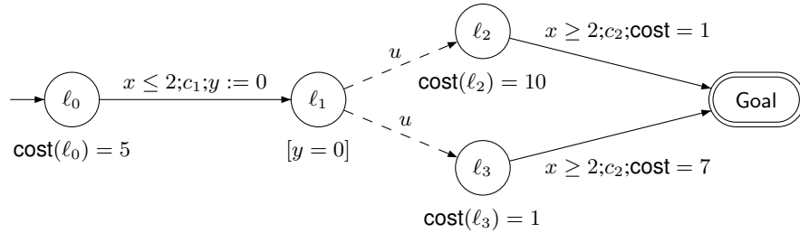
Fig. 1. A Reachability Priced Time Game Automaton A
