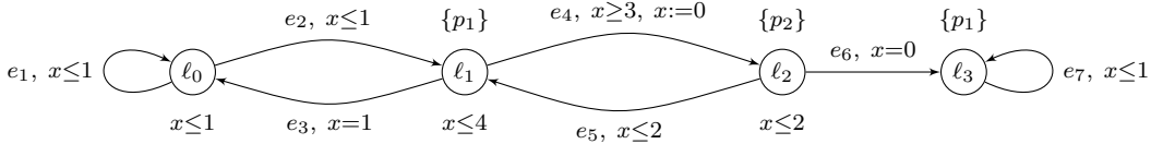
Figure 3: The stochastic timed automaton \mathcal{A}_{\text{running}} .
