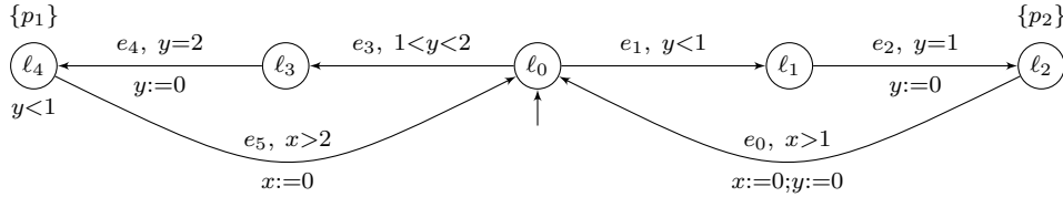
Figure 11: Automaton \mathcal{A}_{\text{unfair}}^2 .
