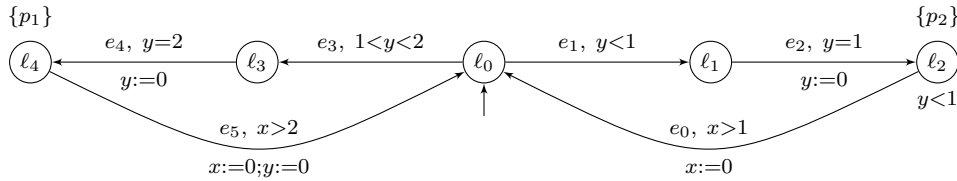
Figure 10: Automaton \mathcal{A}_{\text{unfair}}^1 .
