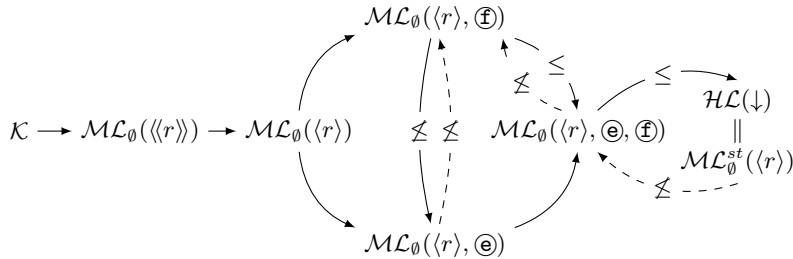
Fig. 1. Different expressive power of memory logics
