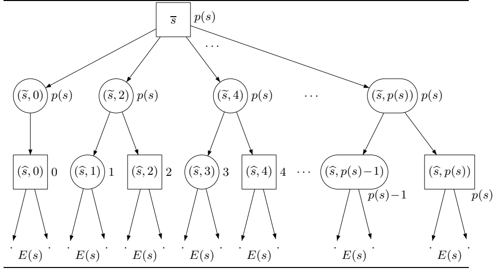
Fig. 1. Reduction gadget when p(s) is even.
